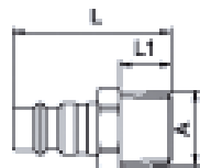
Plug male
